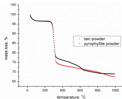
Figure 5. TG curves of talc powder (red dots) and pyrophyllite powder (black dots) in N 2 atmosphere at 15 °C/min heating rate
