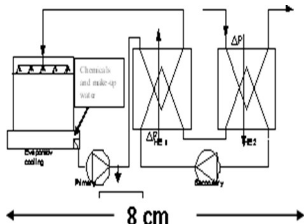
Figure 2. Cooling method with cooling tower loop
